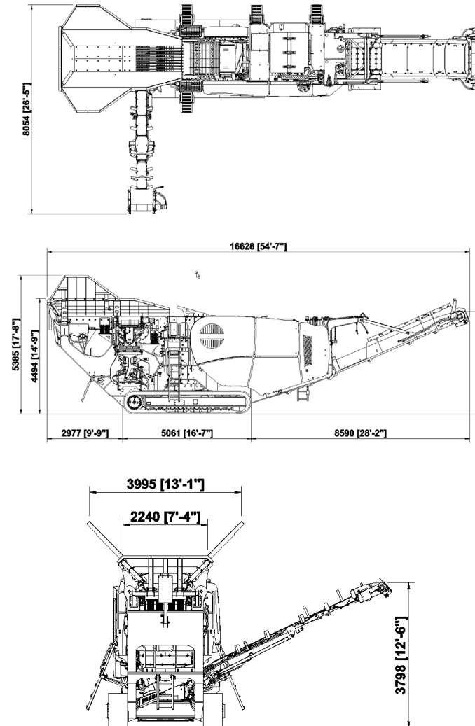
Figure 1: Premiertrak 600 Pre-screen & Bypass Conveyor Working Position
