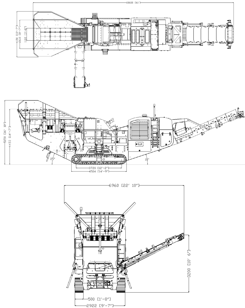
Figure 3: Trakpactor 550 - Pre-screen, Extended Product Conveyor Working Position
