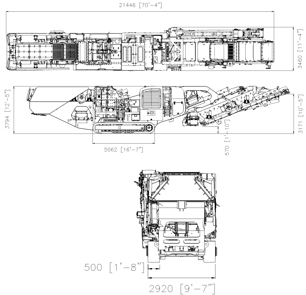
Figure 2: Trakpactor 550SR - Pre-screen, Standard Product Conveyor Transport Position
