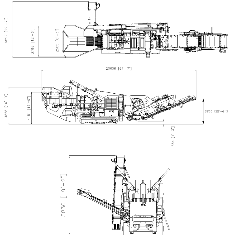
Figure 3: Traktractor 550SR - VGF, Standard Product Conveyor Working Position
