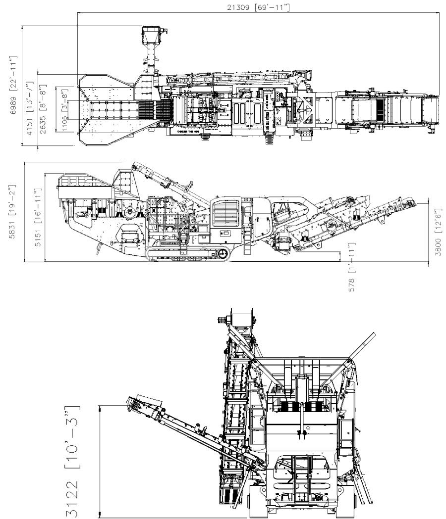
Figure 1: Trakpactor 550SR - Pre-screen, Standard Product Conveyor Working Position
