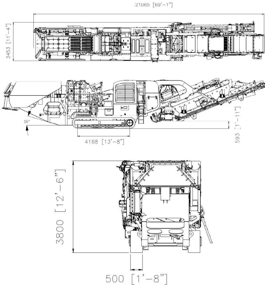
Figure 4: Traktractor 550SR - VGF, Standard Product Conveyor Transport Position
