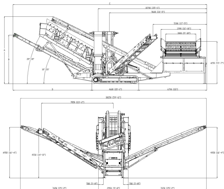
Figure 7: Chieftain 2100X 3 Deck Double Deck Vibrating Grid Standard Length Auxiliary Conveyor - Working Position
