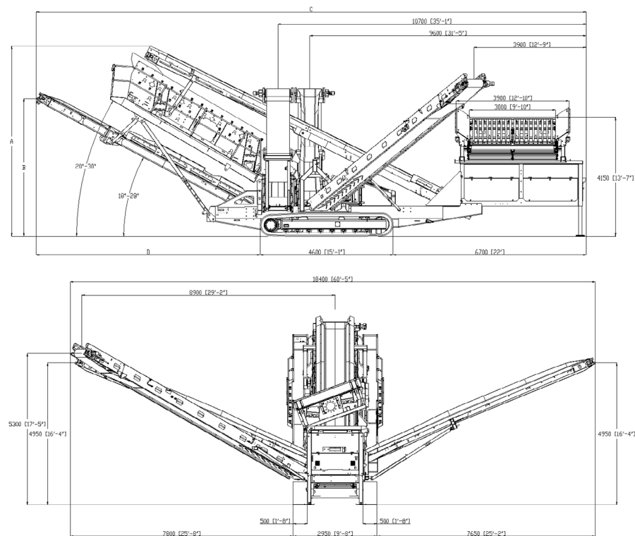
Figure 9: Chieftain 2100X 3 Deck Double Deck Vibrating Grid Extended Length Auxiliary Conveyor - Working Position
