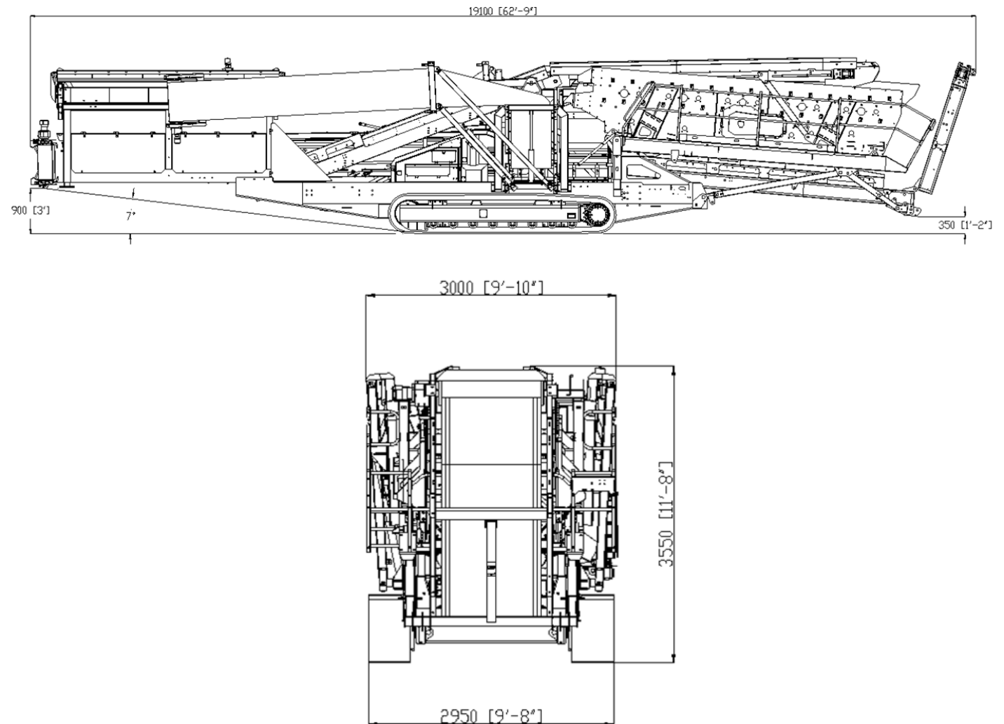
Figure 4: Chieftain 2100X 3 Deck Extended Length Auxiliary Conveyor Transport Position
