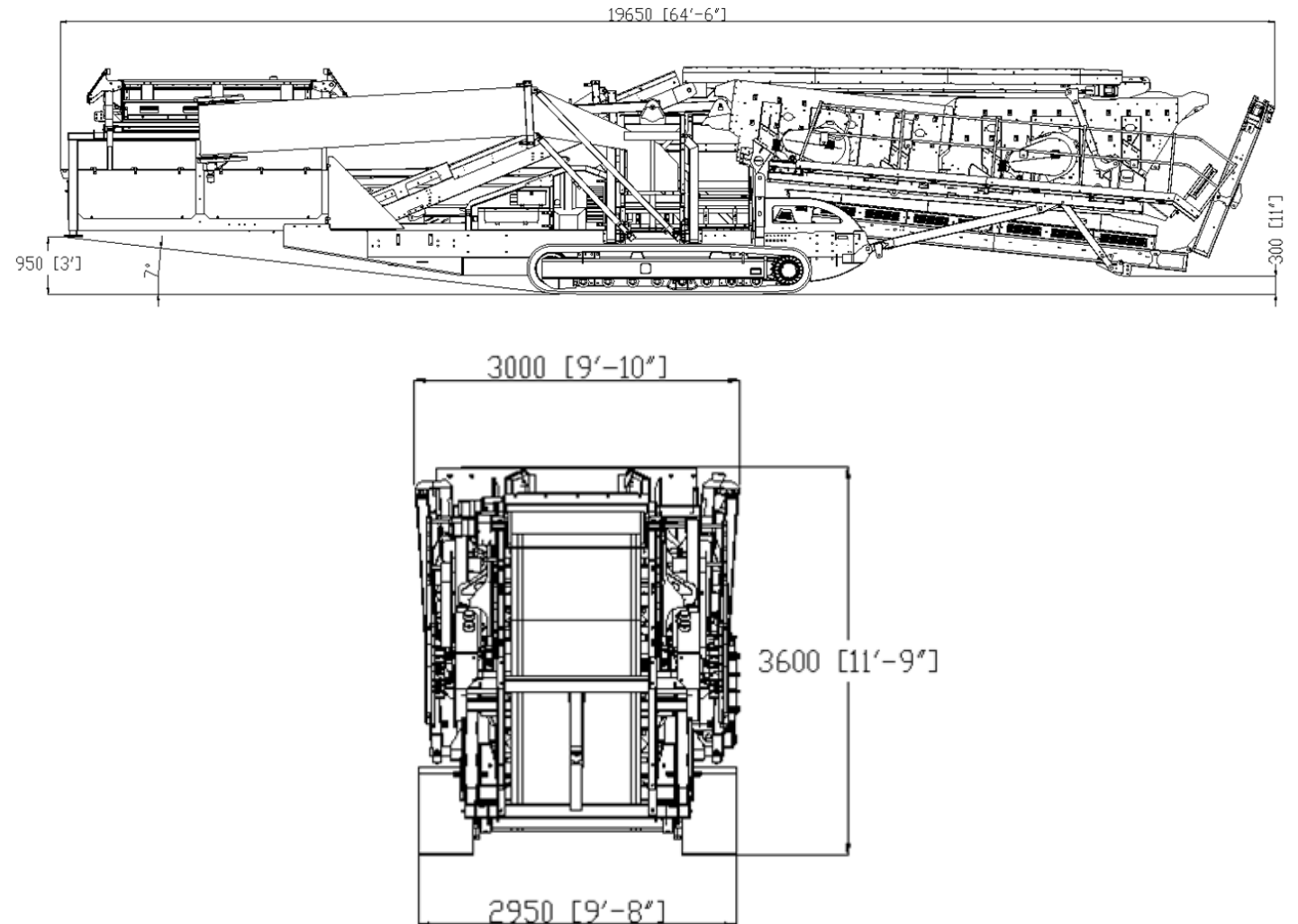
Figure 8: Chieftain 2200 3 Deck Double Deck Vibrating Grid Transport Position
