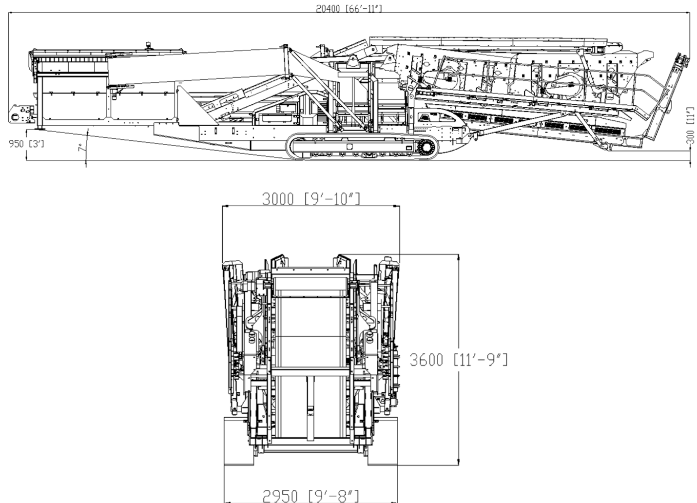
Figure 6: Chieftain 2200 3 Deck Hydraulic Extended Auxiliary Conveyor Transport Position
