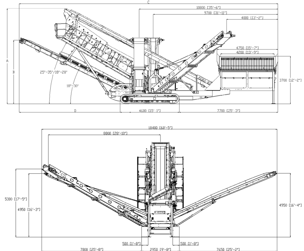
Figure 3: Chieftain 2200 3 Deck Extended Auxiliary Conveyor Working Position
