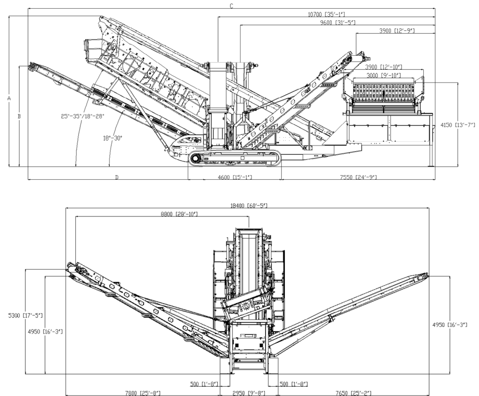
Figure 9: Chieftain 2200 3 Deck Extended Auxiliary Conveyor Double Deck Vibrating Grid Working Position
