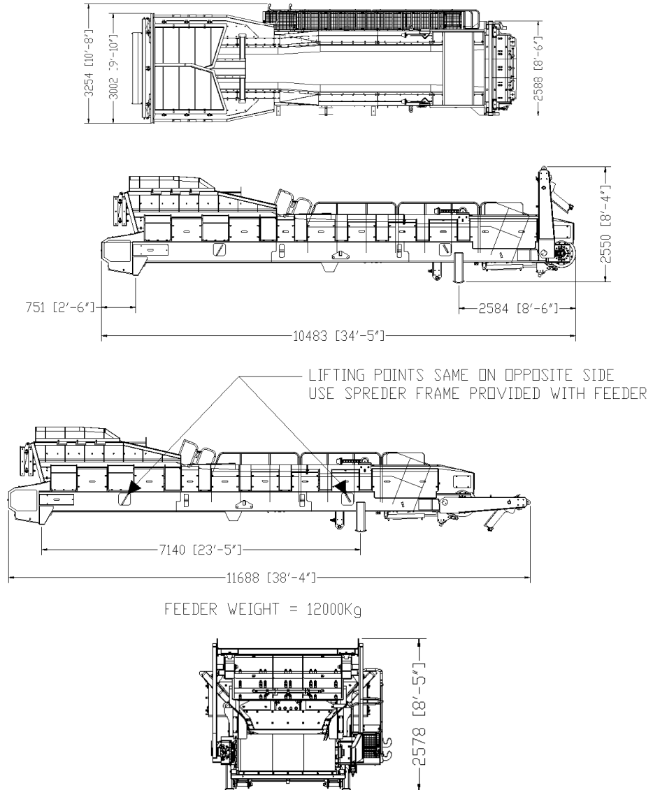
Figure 3: 1500 Maxtrak Transport Position
