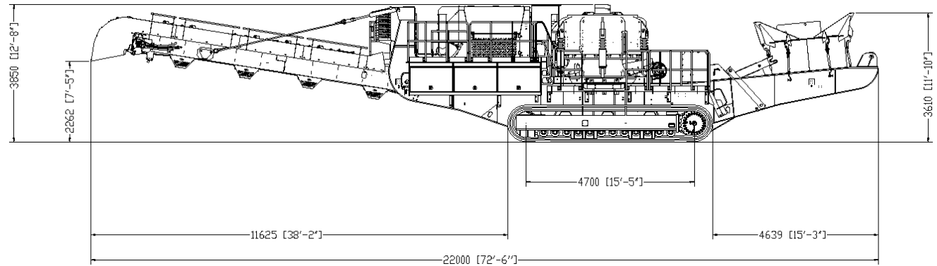
Figure 2: 1500 Maxtrak Transport Position
